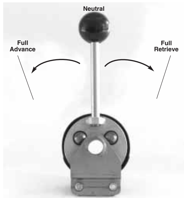
Figure 7 – Autofeed
